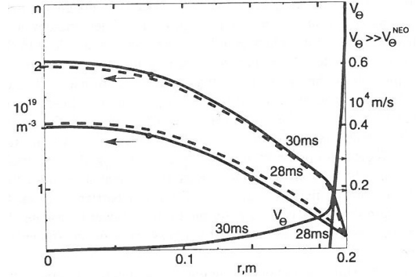
Fig. 3 Scenarios of two LH transitions. Full curves are transitions triggered by poloidal rotations, broken curves are transitions triggered by density depletions with poloidal rotation imposed to zero.
