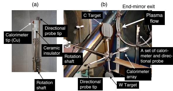
FIG. 4. Photograph of the diagnostics. (a) Calorimeter and directional probe. (b) Rotatable target plates.
