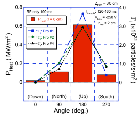
FIG.5. Angular dependence of ion flux and that of heat flux by rotating the diagnostic instrument.
