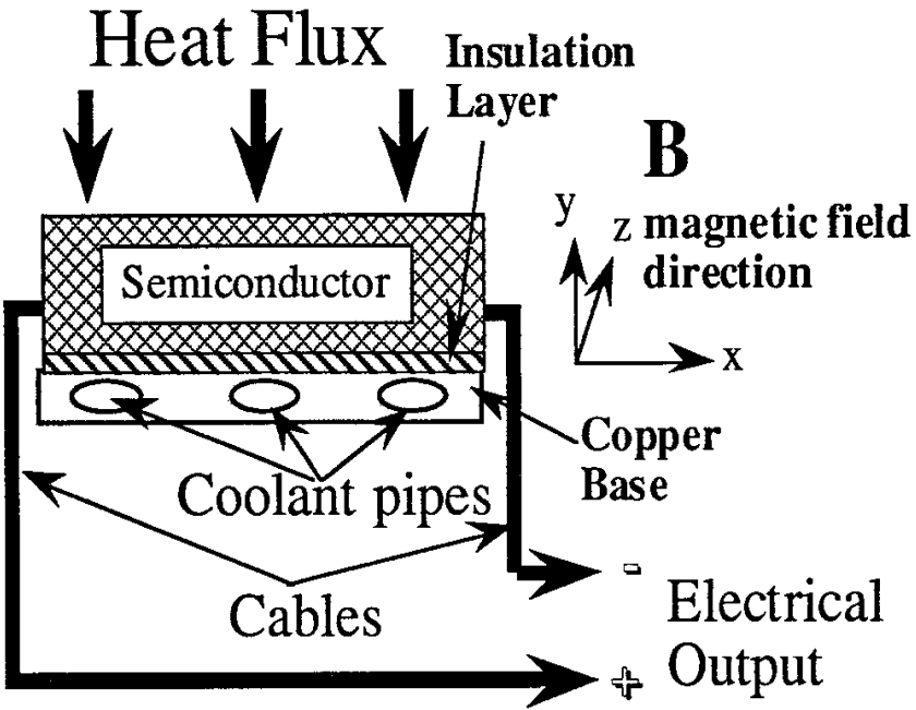
Fig. 9. Schematic configuration of the heat conversion device using the Nernst effect.
