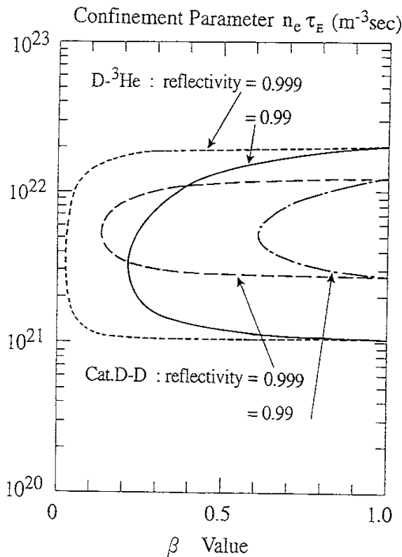
Fig. 6 Ignition condition with parameter of wall reflectivity.
