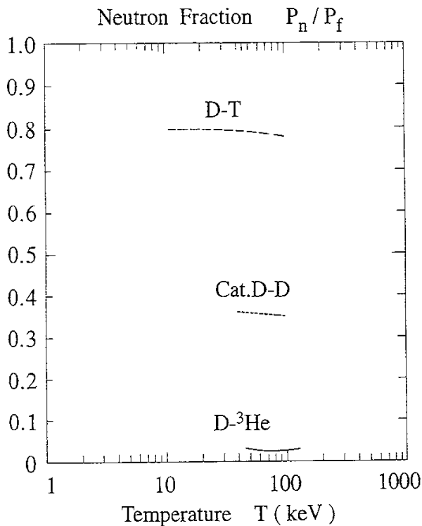
Fig. 2 Fraction of neutron power in fusion power.
