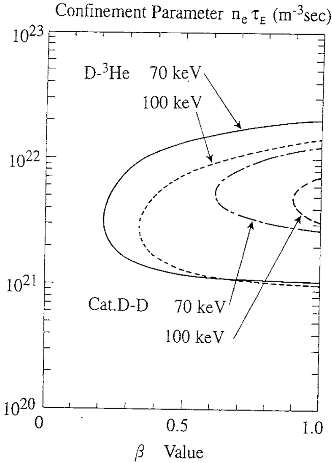
Fig. 3 Ignition condition for catalyzed D-D and D- 3 He reactors at \eta_{\text{ash}} \equiv \tau_{\text{ash}}/\tau_E = 2 as a function of \beta value.
