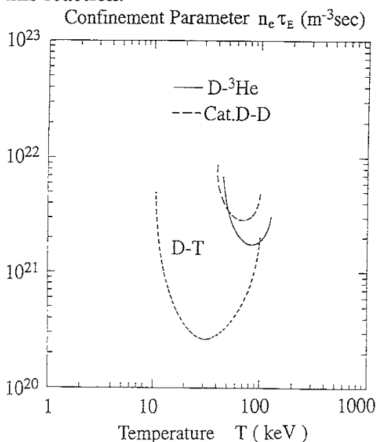
Fig. 1 Ignition conditions for D-T, catalyzed D-D and D- ^3\text{He} concepts.
