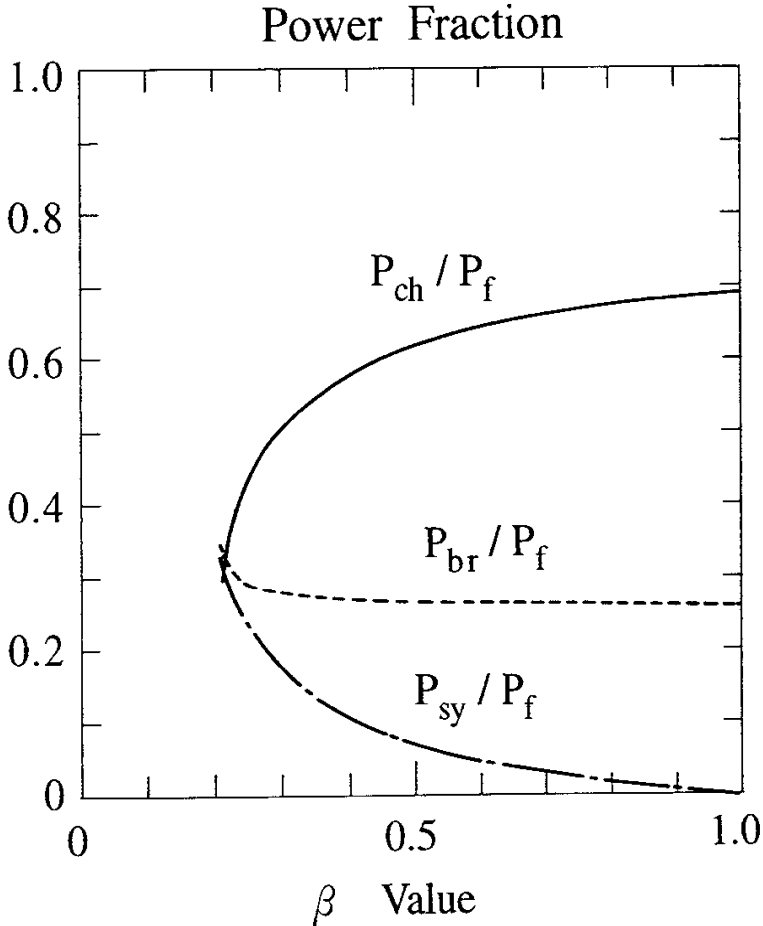
Fig. 4 Calculated power fraction for D- ^3\text{He} at T_e = 70 keV and \eta_{ash} \equiv \tau_{ash} / \tau_E = 2 .
