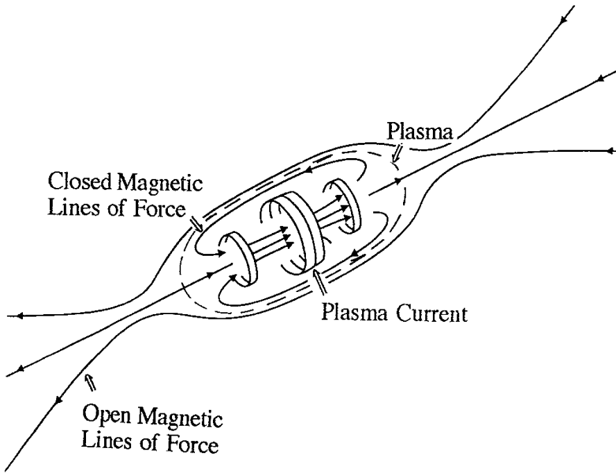
Fig. 5 Schematic drawing of FRC.
