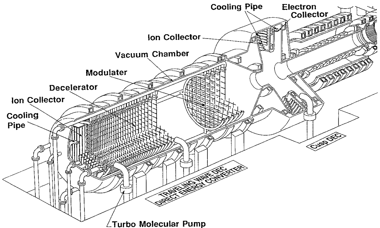
Fig. 7 Schematic view of Cusp DEC and TWDEC.
