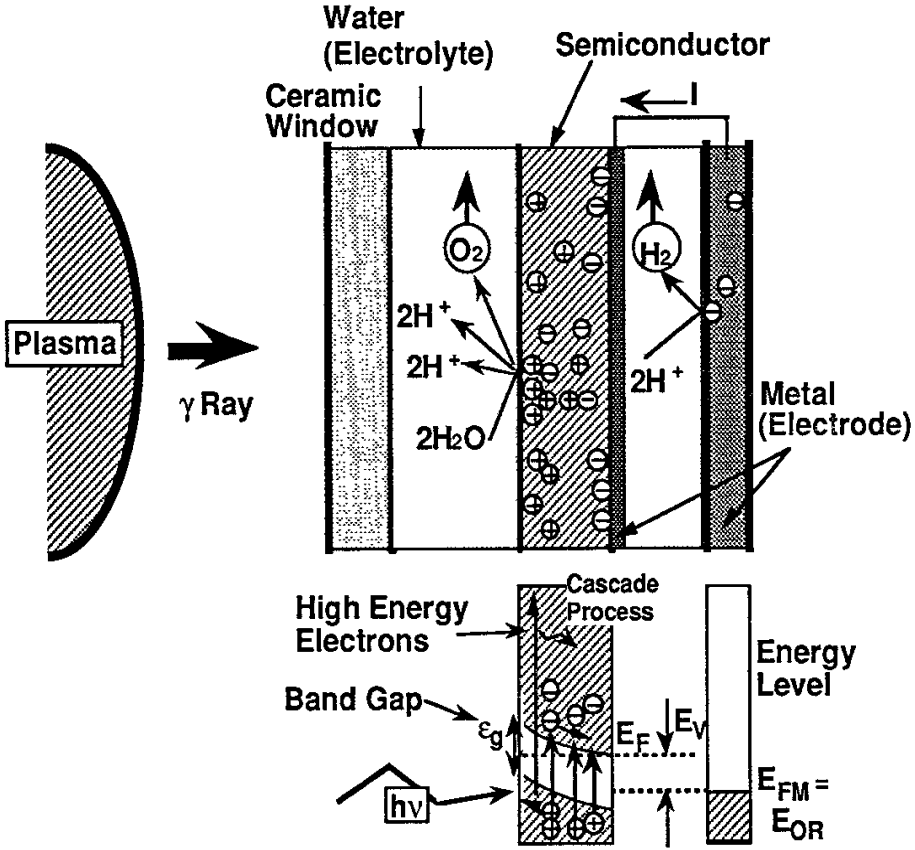
Fig. 8 Principle of direct hydrogen production by \gamma rays.
