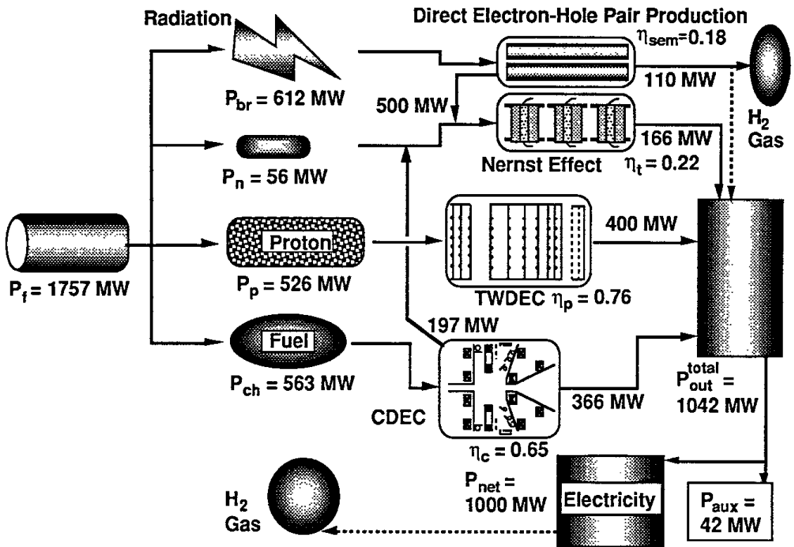
Fig. 11 Power flow for ARTEMIS-L having 1 GW electricity output.
