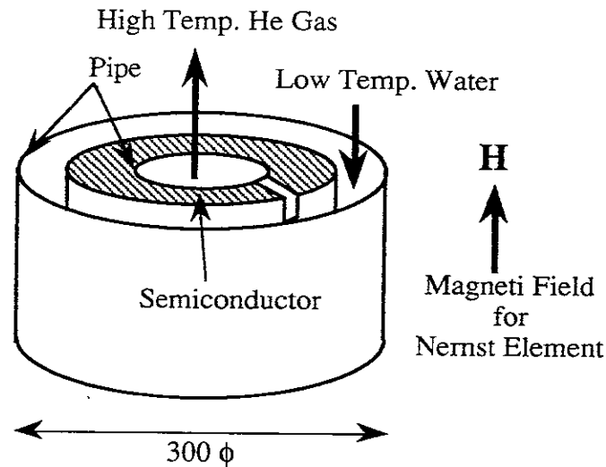
Fig. 5 Schematic structure of energy conversion pipe
