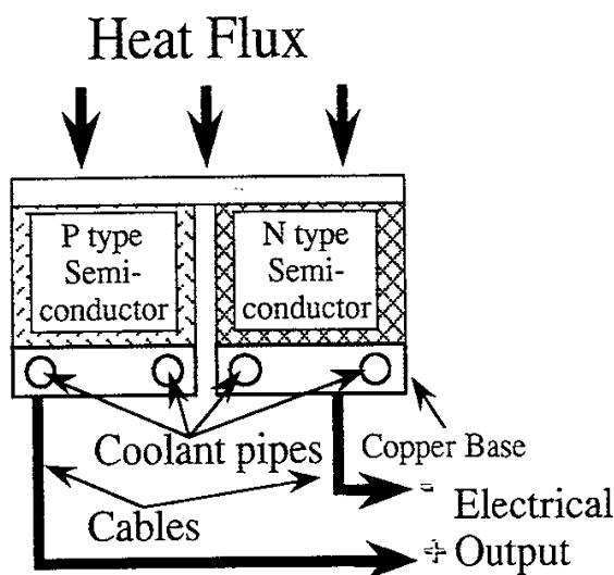
Fig. 1 Set up of thermoelectric element
