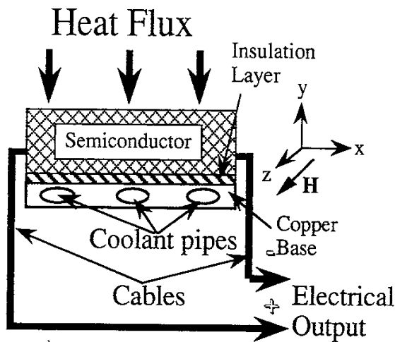
Fig. 2 Set up of Nernst element
