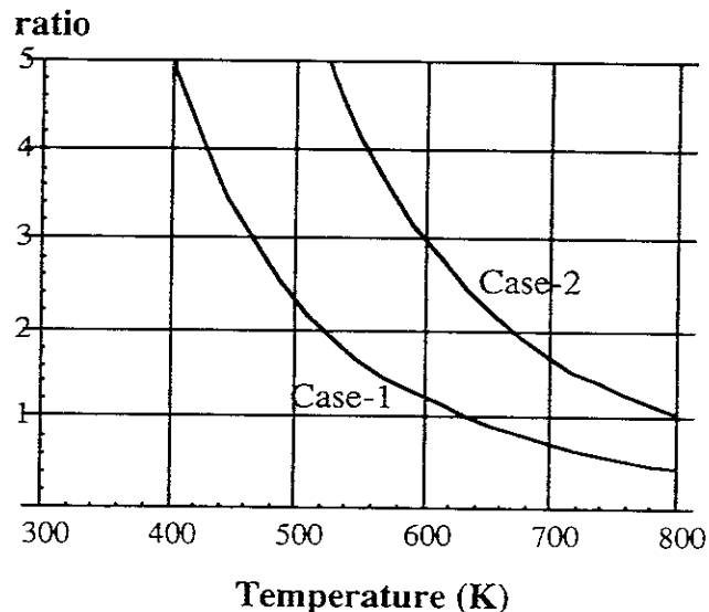
Fig. 3 Ratio of Thermoelectric and Nernst Elements
