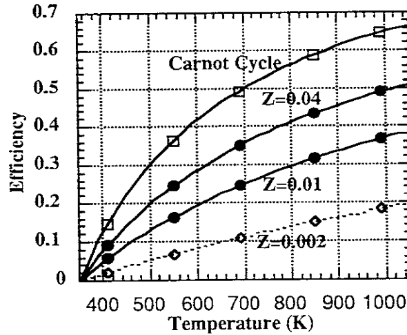
Fig. 4 Efficiency of Carnot cycle, Z=0.002 , Z=0.01 , Z=0.04 for low temperature of 350 K.
