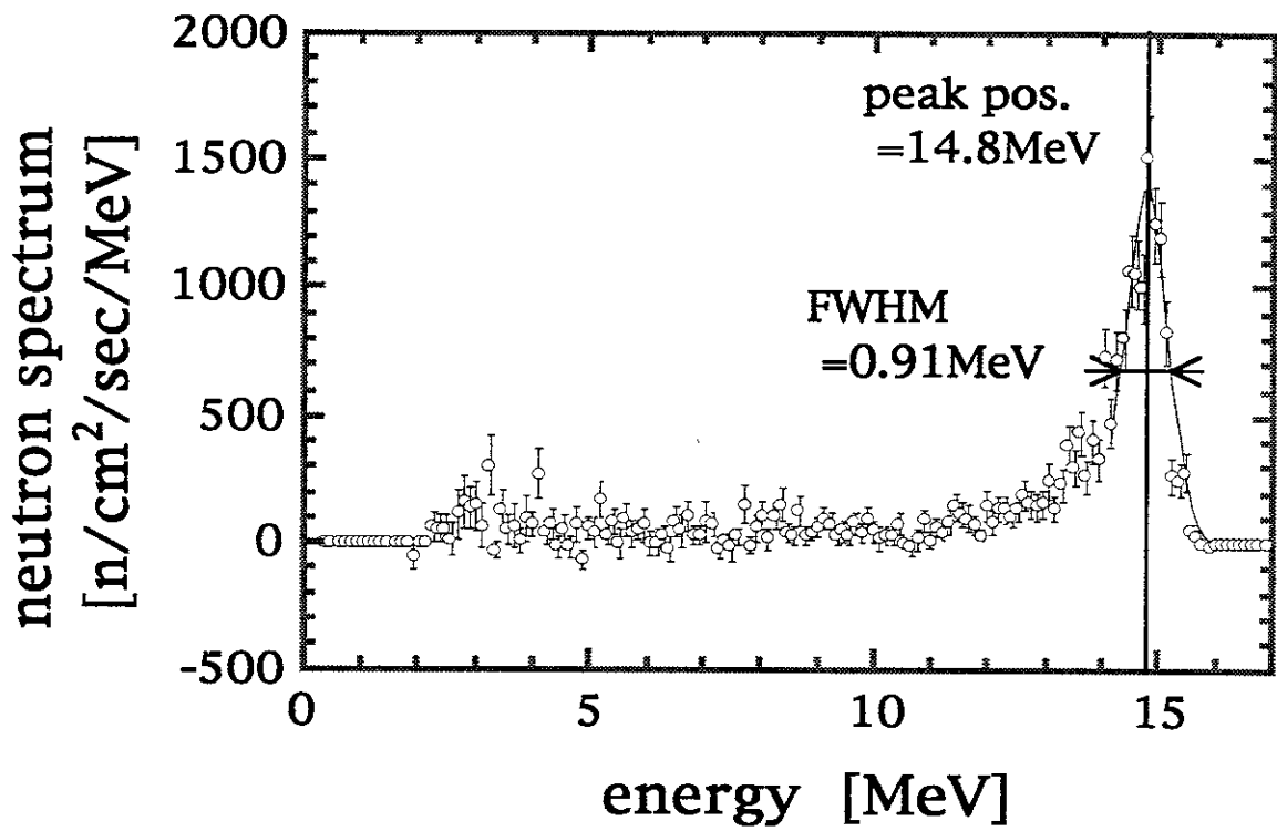
Fig. 2-9 Obtained neutron spectrum for D-T neutron at the calibration experiment of the prototype
