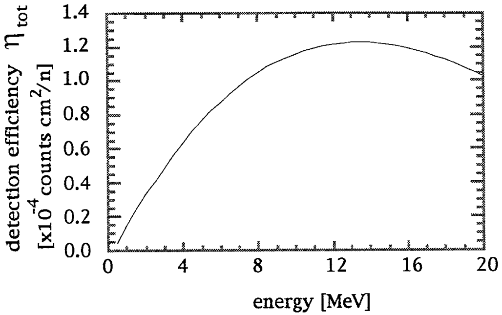
Fig. 2-10 Calculated detection efficiency : \eta_{tot} [counts/(n/cm 2 )] of the prototype spectrometer. The loss of events due to the walk of signals from \Delta E -detector is considered in the calculation.
