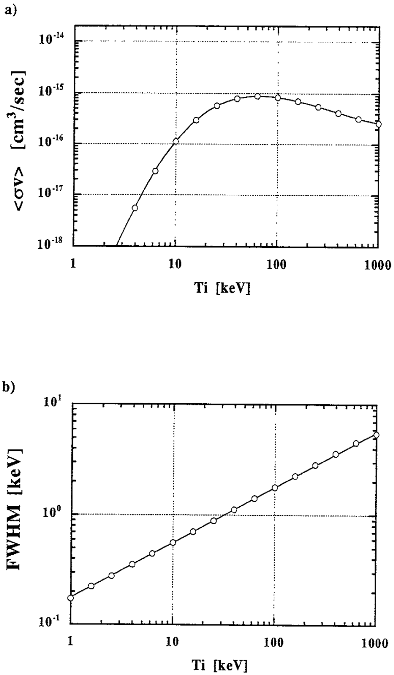
Fig.4-3 (a) Fusion reactivity, and (b) FWHM of the D-T neutron peak are calculated for D-T Maxwellian plasmas. The open circles show the result of NESFP, and the solid line denotes that in references.
