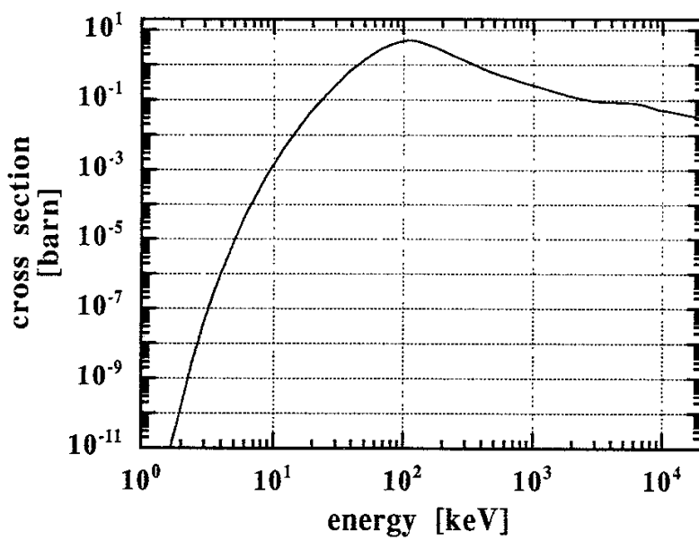
Fig. 4-1 D-T fusion cross section used in the NESFP code[1].
