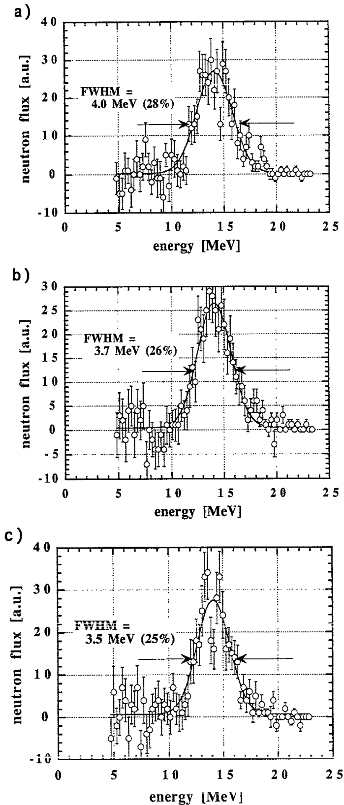
Fig.5-3 Energy spectra of neutron obtained for NBI and ICRF heated plasma. (a) and (b) are that obtained for discharges with ^3\text{He} minority. (c) is that obtained for a discharge without ^3\text{He}
