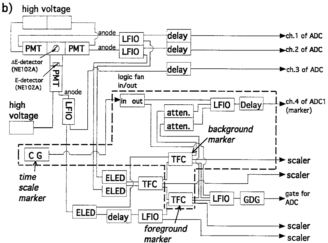
Fig. 3-2 Block diagram for COTETRA (a)set-A and (b)set-B on TFTR. The modules surrounded by the dashed lines are newly applied for TFTR experiments. The labels shown in these figures are; PMT: photo multiplier tube, SSBD: silicon surface barrier detector, DBS: detector bias supply, CG: clock generator, ELED: extrapolated leading edge discriminator, LFIO: linear fan in and out, TFC: two fold coincidence, GDG: gate and delay generator, atten.: attenuator.
