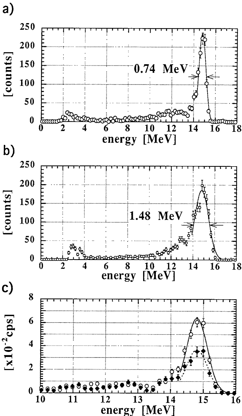
Fig. 2-13 (a) Energy spectra obtained at the calibration experiment for set-A, and (b) that for set-B. Raw data are shown by open circles in these figure. Lines show results of the gaussian fitting with the fitting region of above 14.3-MeV for set-A and 13.9-MeV for set-B. (c) A spectrum for set-A when a polyethylene block is placed in front of the \Delta E -detector, shown by closed diamonds, are compared to the spectrum without the block, shown by open circles. The neutron source intensity is almost same in each case and each spectrum is normalized with the measurement time. The solid line shows the fitting of open circles to gaussian curve and the dashed line shows that of closed diamonds.
