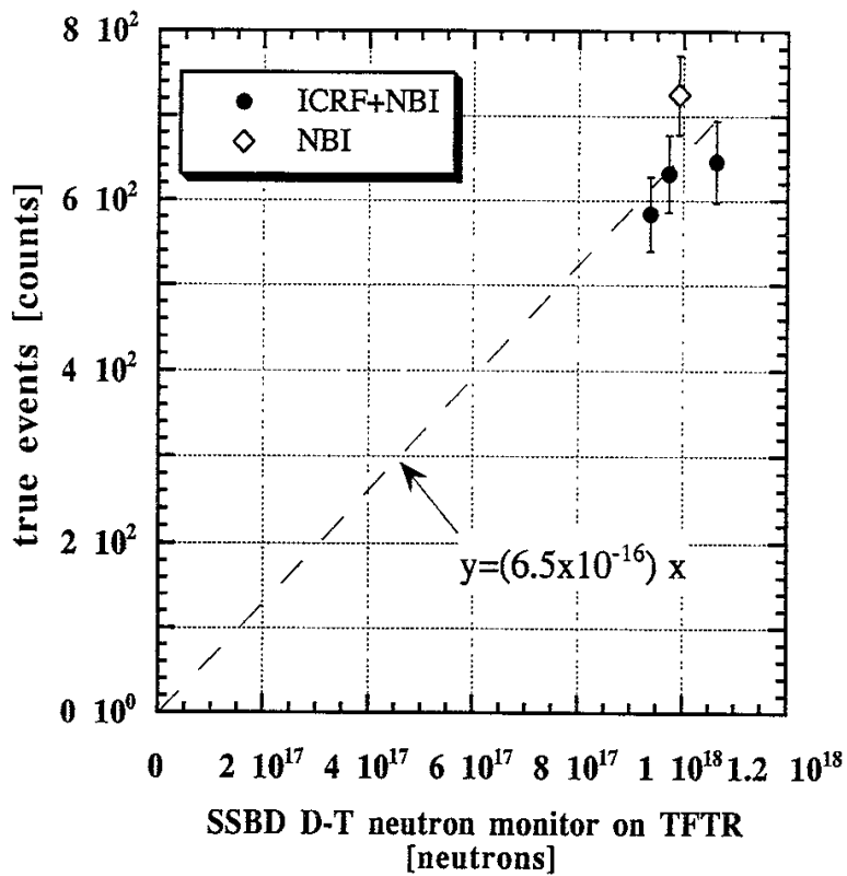
Fig.3-6 Total counts of COTETRA set-B vs. D-T neutron yield of TFTR obtained by Si-diode
