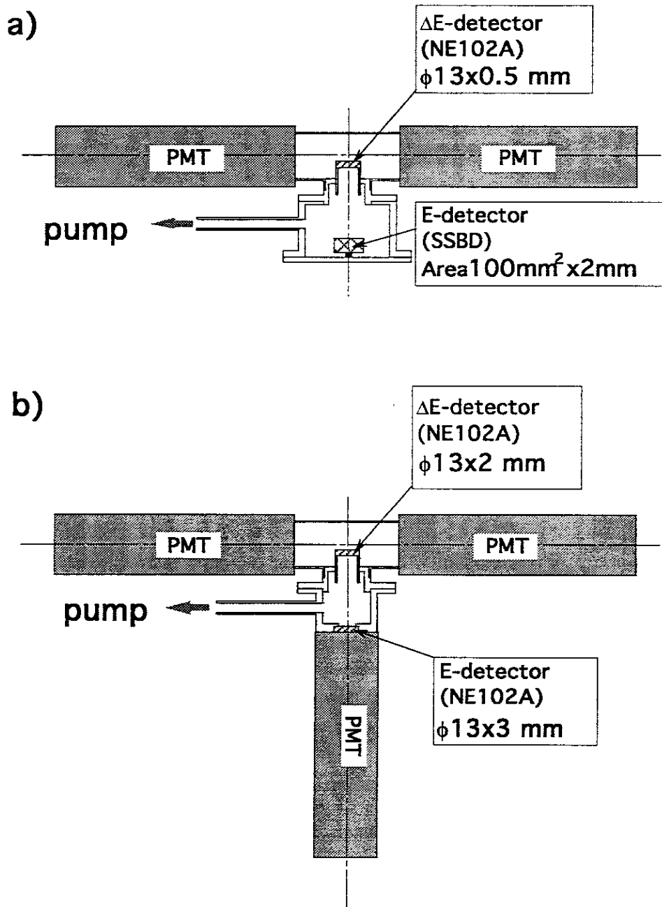
Fig.2-11 Schematic drawings of COTETRA for TFTR D-T experiments. (a) Set-A has better energy resolution, and (b) set-B has better counting rate capability and detection efficiency.
