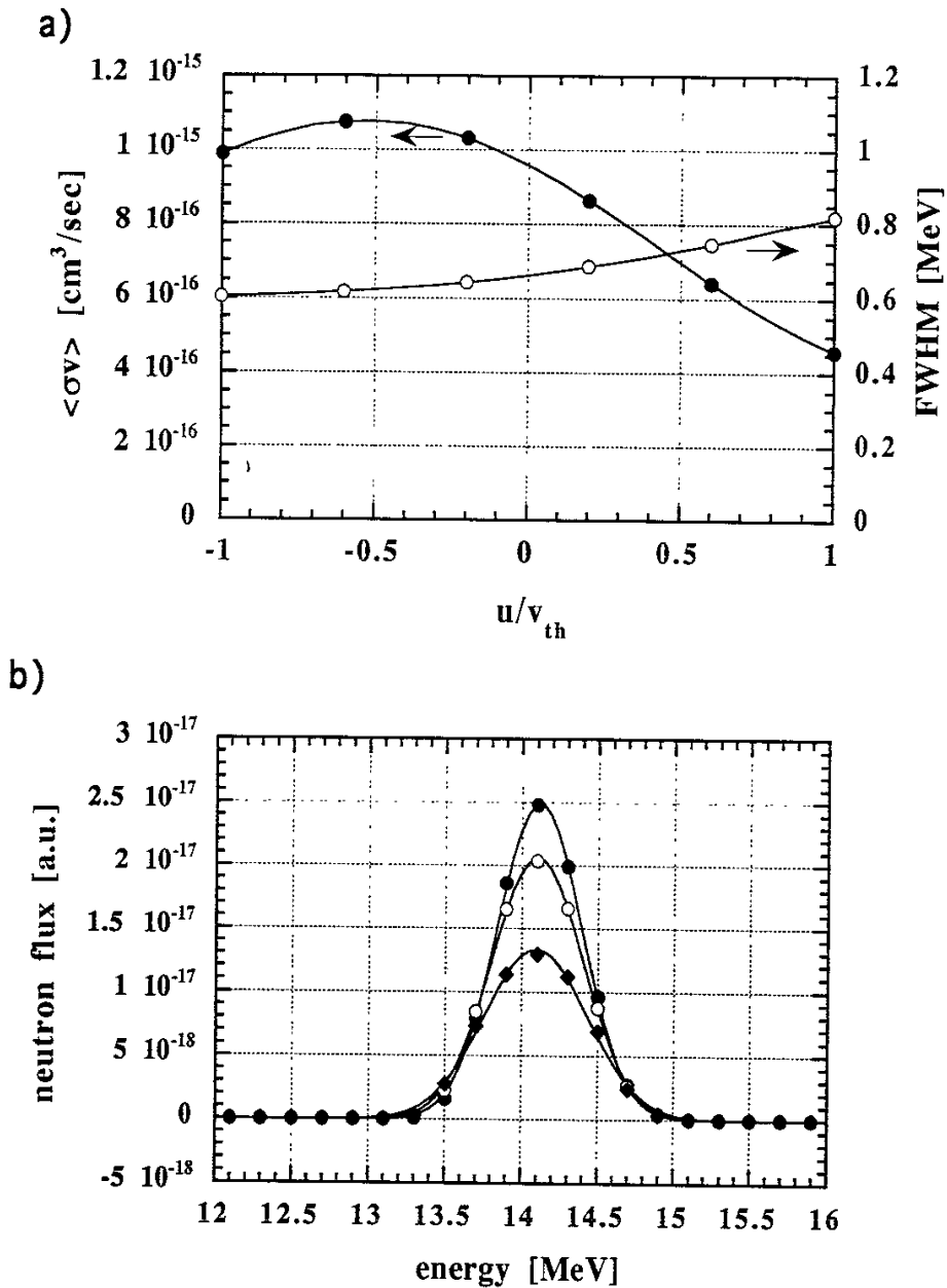
Fig.4-4 Result of the NESFP calculation for the case in which the mono-energetic tritium ions are injected parallel to magnetic field lines into the thermal deuterium ion plasma drifting parallel to the lines. The deuterium temperature were assumed to be 30keV. The sign of x-axis shows the drift direction of deuterium ions with respect to the tritium beam direction. It was set to minus when deuterium ions are moving in the counter-direction to tritium ions, and to plus in the co-direction. (a) The line with closed circles shows the calculated \langle \sigma_a v_c \rangle , and that with open circles does the FWHM of D-T neutron peak. (b) The example of the calculated D-T neutron spectra for u/v_{th} = -0.5 (closed circles), 0 (open circles), and 0.5 (closed diamonds).
