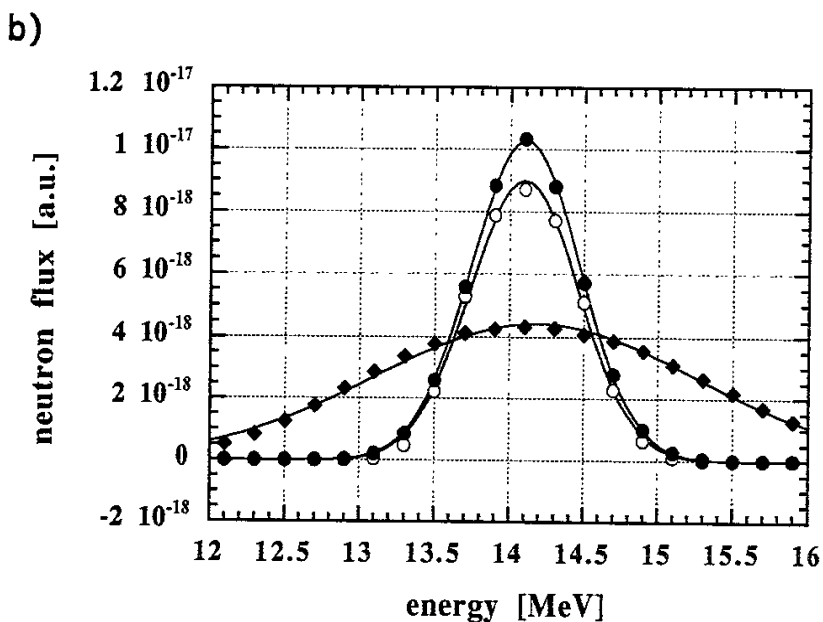
Fig.4-5 Result of the NESFP calculation for the case in which the velocity distribution of deuterium ions is an isotropic Maxwellian of a temperature 30keV, and that of tritium ions is anisotropic Maxwellian, i.e., the tritium ion was assumed to have different temperature in the direction perpendicular to magnetic field line and in the parallel direction. The parallel temperature was assumed to be 30keV, and the perpendicular temperature was varied in the calculation. (a) The line with closed circles shows calculated \langle \sigma_{av} \rangle , and that with open circles does the FWHM of D-T neutron peak. (b) The example of the calculated D-T neutron spectra for T_i^{\text{DTP}}=40\text{keV} (open circles), 160keV(closed circles), and 400keV(closed diamonds).
