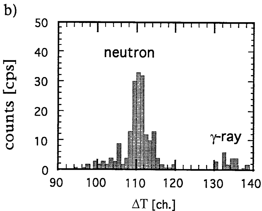
Fig. 2-6 TOF spectra of neutrons and \gamma -rays which flew to \Delta E -detector from tritium target at the calibration experiment of the prototype. The \Delta T is the time difference between the \Delta E -detector signal and the delayed accelerator's pick-up ring. Events due to fast particles appear right hand side of the figures. (a) spectrum obtained for foreground run. (b) that obtained for background run.
