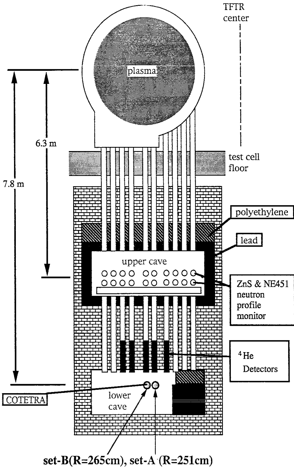
Fig. 3-1 Schematic drawing of multi-channel neutron collimator (MCNC) at Bay-K on TFTR. ZnS and NE451 detectors are installed in the upper cave. 4 He proportional counters are installed in the flight tube between upper and lower cave. Set-A of COTETRA is installed in the lower cave under channel #5 and set-B is under channel #6 of the MCNC. These channel correspond to the major radius of 251cm and 265cm, respectively.
