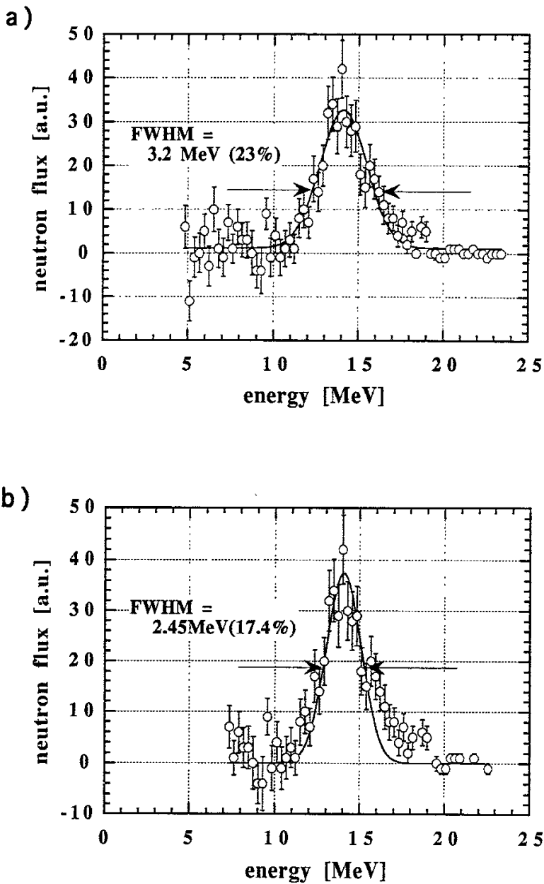
Fig.5-1 Energy spectrum obtained for a NBI heated D-T plasma. (a) open circles show the obtained spectra during the discharge, and the solid line shows the gaussian fitted curve of them. (b) open circles are the same spectrum as shown in (a), but the data point whose error is equal to zero were eliminated. Solid line is obtained by a fitting of gaussian curve whose FWHM are fixed to 17.4%.
