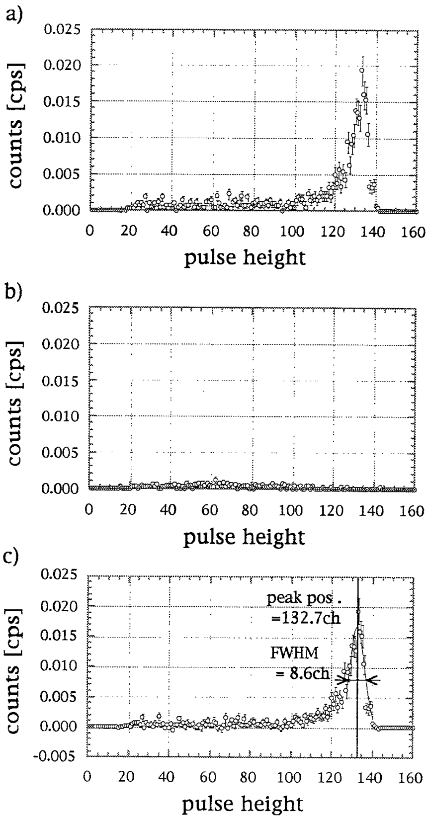
Fig. 2-7 One dimensional pulse height spectra of neutrons for (a) foreground run, (b) background run and (c) true events. Both in (a) and (b), the \gamma -ray events are already removed. The PHS (c) is obtained by subtracting the PHS (b) from (a).
