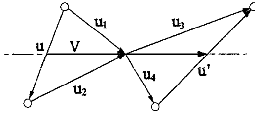
Fig.C-1 Nuclear reaction between particles kind "1" and "2". As a result of the reaction, particles kind "3" and "4" are emitted.
