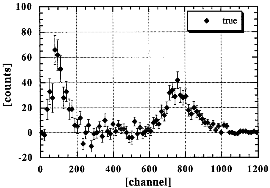
Fig. 3-7 Pulse height spectra for (a) foreground and background events, and (b) true events which were obtained by subtraction of background PHS from foreground PHS. These PHS were obtained for an NBI-discharge.
