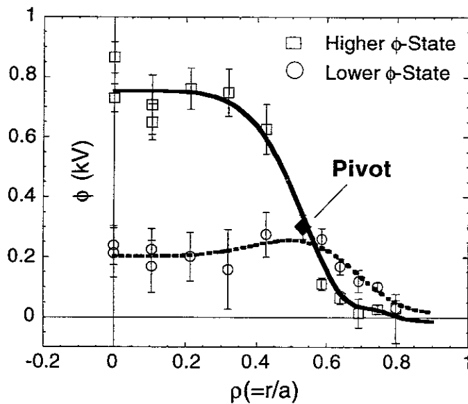
FIGURE 2: Potential profiles of higher and lower states. Here \rho is the normalized minor radius. The change of potential profile is seen even in the periphery.
