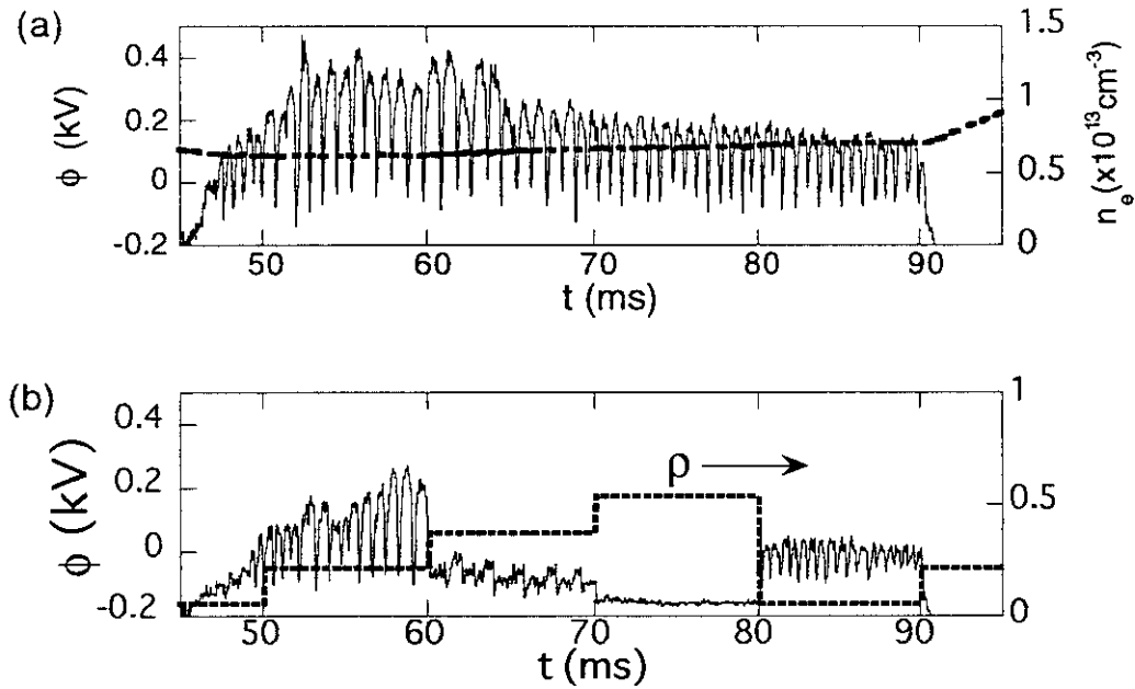
FIGURE 3: An example of long-term electric pulsation. In this case, the electron density is rather higher about n_e \sim 7 \times 10^{12} \text{ cm}^{-3} , and the pulsation regime is confined to inside of \rho = 0.5 . (a) Time evolution of potential near the center and line averaged electron density. (b) Time evolution of potential. The observation point of potential alters in 10ms step; \rho = 0.21 (50-60ms), \rho = 0.37 (60-70ms), \rho = 0.53 (70-80ms) and \rho = 0.05 (80-90ms).
