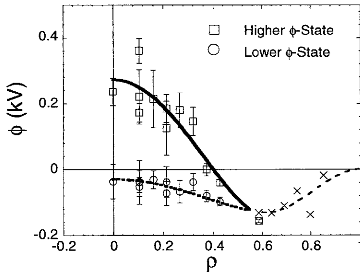
FIGURE 4: Potential profiles of higher and lower potential states are shown in case of electric pulsation with lower density. Outside of \rho = 0.53 , no change is seen during the pulsation. The data represented by the \times -marks is taken in radial scans.
