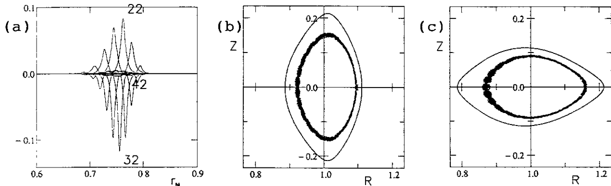
Fig. 3 The same quantities as in Fig. 1 for n \sim M in a helicity-dominant equilibrium.
