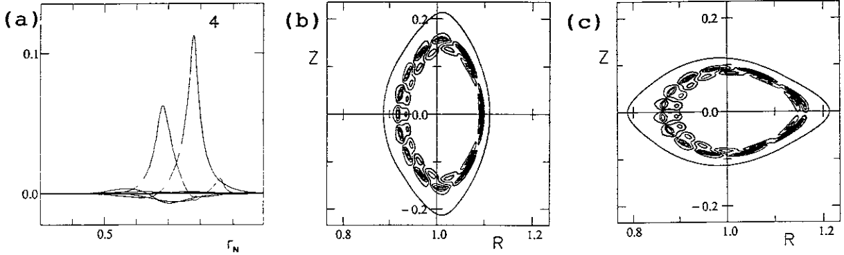
Fig. 1 (a) \vec{\xi} \cdot \nabla \psi vs. r_N (normalized radial coordinate) with the dominant toroidal mode number, and the corresponding contours of \tilde{P} = -\nabla P \cdot \vec{\xi} on the vertically (b) and horizontally (c) elongated poloidal cross sections.
