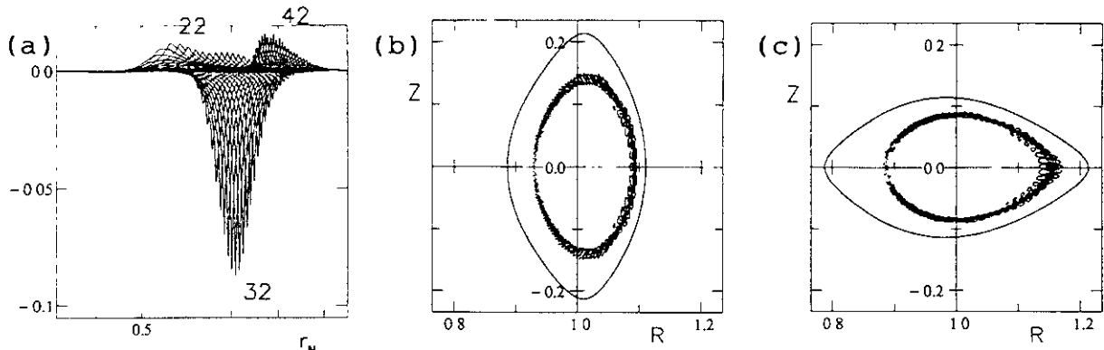
Fig. 2 The same quantities as in Fig. 1 for n \sim M in a toroidicity-dominant equilibrium.
