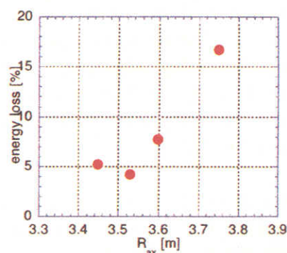
FIG. 8. R_{ax} dependency of NBI heating energy loss rate by orbit loss evaluated by GNET
