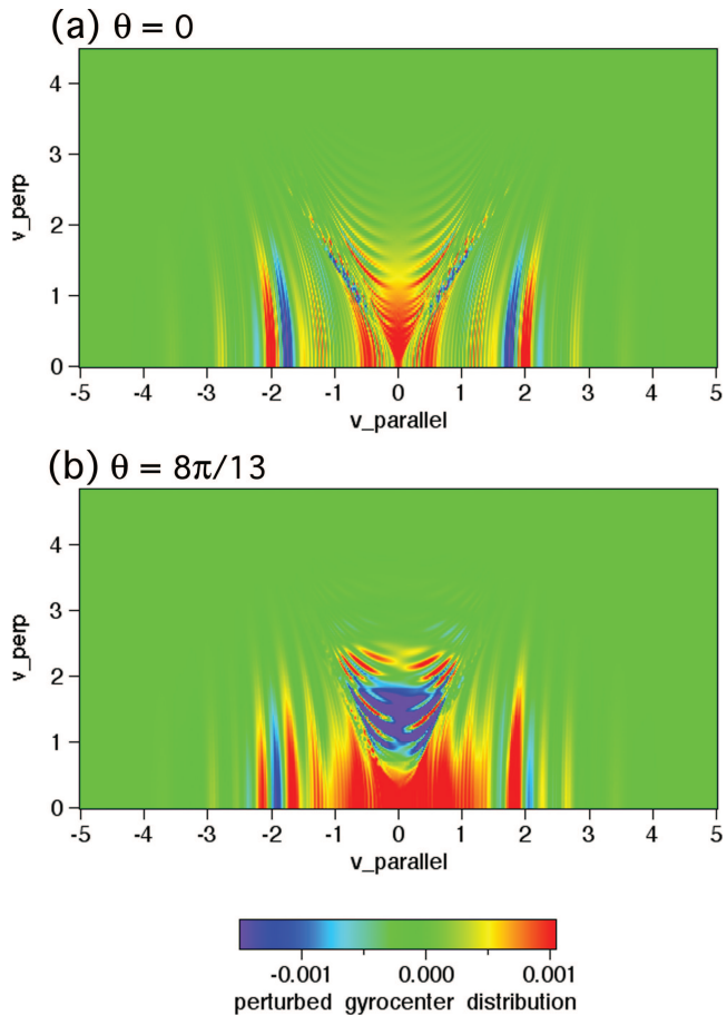
FIG. 3: Structures of the real part of the perturbed ion gyrocenter distribution function \delta f_{ik_{\perp}}^{(g)} on the (v_{\parallel}, v_{\perp}) -space obtained by the simulation at t = 12.5(R_0/v_{ti}) for the case of the helical system in Fig. 1 (b). The parallel and perpendicular velocities are both normalized by v_{ti} \equiv (T_i/m_i)^{1/2} . Here, (a) and (b) are plotted for (\theta, \zeta) = (0, 0) and (\theta, \zeta) = (8\pi/13, 12\pi/13) , respectively, in which the former corresponds to the the minimum of the magnetic field strength within the flux surface and the latter locates the bottom of the local helical ripple with helical-ripple-trapped particles having relatively large radial drift velocities.
