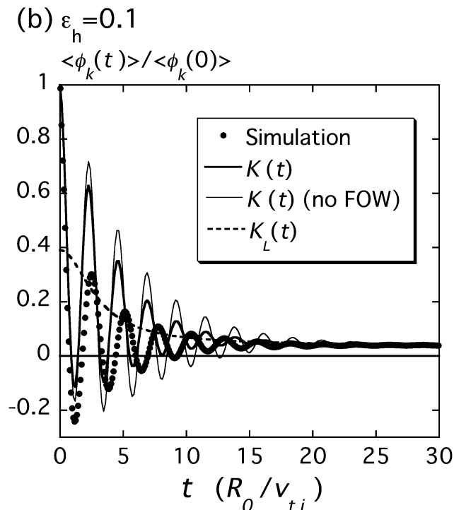
FIG. 1: Time evolution of the zonal-flow potential obtained by the simulations for the tokamak case ( \epsilon_h = 0 ) (a) and for the helical system ( \epsilon = 0.1 ) (b). In both cases, q = 1.5 and k_r a_i = 0.131 are used. The simulation results are plotted by solid circular symbols. Thick solid curves represent the response kernel \mathcal{K}(t) obtained by Eq. (63) with the use of Eqs. (18), (57) and the complex-valued GAM frequency \omega = \omega_G + i\gamma calculated by numerically solving 1/\mathcal{K}_{GAM}(\omega) = 0 where \mathcal{K}_{GAM}(\omega) is defined by Eq. (14). Thin solid curves represent the response kernel \mathcal{K}(t) obtained by neglecting the FOW effect when calculating (\omega_G, \gamma) . The response kernel \mathcal{K}_L(t) given by Eq. (57) is also plotted by dashed lines.
