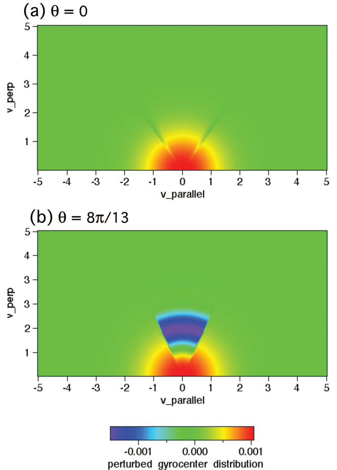
FIG. 4: Structures of the real part of the perturbed ion gyrocenter distribution function \delta f_{ik_{\perp}}^{(g)} on the (v_{\parallel}, v_{\perp}) -space obtained from the analytical solution given by Eqs. (64) and (65) at t = 12.5(R_0/v_{ti}) for the case of the helical system in Fig. 1 (b). Here, (a) and (b) correspond to the cases of Figs. 3 (a) and (b), respectively.
