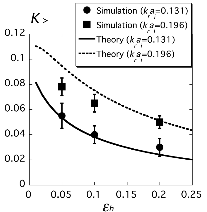
FIG. 2: The long-time limit of the response kernel \mathcal{K}_> as a function of \epsilon_h for k_r a_i = 0.131, 0.196 , and \epsilon_t = 0.1 . The simulation results and the theoretical formula in Eq. (59) are represented by symbols with error bars and curves, respectively.
