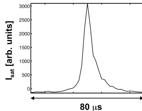
FIG. 8 Conditional averaging result of the I_{sat} of Fig. 2 (b).
