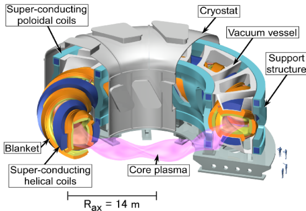
FIG. 1. Helical-type power reactor FFHR2m1.
