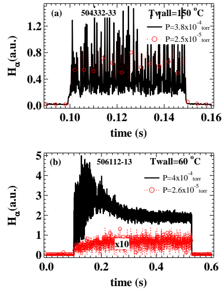
Fig.6 The waveform of H_\alpha intensities taken at initial phase (a) and middle phase (b) in the experimental campaign. Data are compared at two pressures of 2.5\times 10^{-5}\text{-}4\times 10^{-4} torr.
