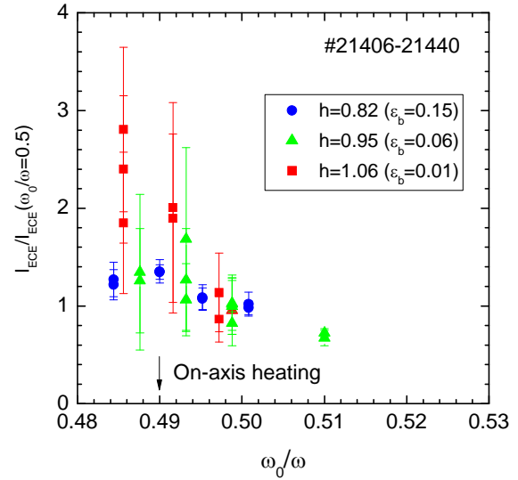
FIG 5. Dependence of ECE intensity on magnetic field strength. The intensity is normalized by that at \omega_0/\omega=0.5 for each configuration. The electron density range is 0.3\text{-}0.6 \times 10^{19} \text{ m}^{-3} .
