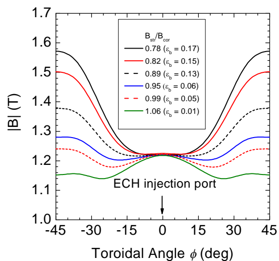
FIG. 1. Magnetic field profile along magnetic axis in Heliotron J. The bumpiness is scanned from \varepsilon_b=0.01 to 0.17, enabling ripple top and ripple bottom heatings.
