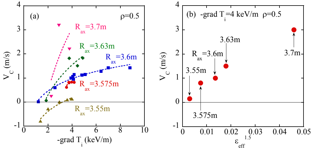
FIG.4. (a) Dependences of convection velocity of carbon on the ion temperature gradient in the plasma with different magnetic axis position. (b) The convection velocity when the ion temperature gradient is -4\text{keV/m} plotted as the function of effective ripple strength.
