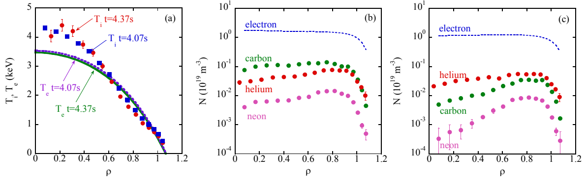
FIG. 5. (a) Radial profiles of ion temperature and electron temperature. Radial profiles of electron, helium, carbon, and neon density (b) before and (c) after the impurity hole developed.
