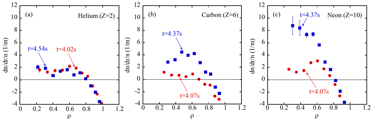
FIG. 6. Radial profiles of normalized density gradient of (a) helium, (b) carbon, and (c) neon profile before and after the impurity hole developed.
