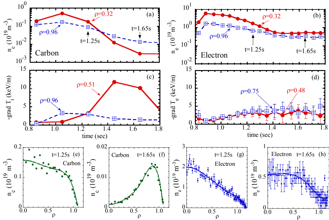
FIG.2. Overview of the discharge with the impurity hole from Ref.[3]. Time evolutions of (a) carbon density, (b) electron density, (c) ion temperature gradient, and (d) electron temperature gradient. Radial profiles of carbon density (e) before and (f) after the impurity hole developed. Radial profiles of electron density (g) before and (h) after the impurity hole developed.
