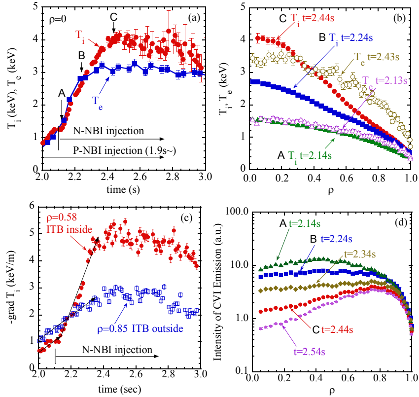
FIG. 1. (a) Time evolution of ion temperature and electron temperature. (b) Radial profiles of ion temperature and electron temperature. (c) Time evolution of ion temperature gradient. (d) Radial profiles of charge exchange emission of carbon.
