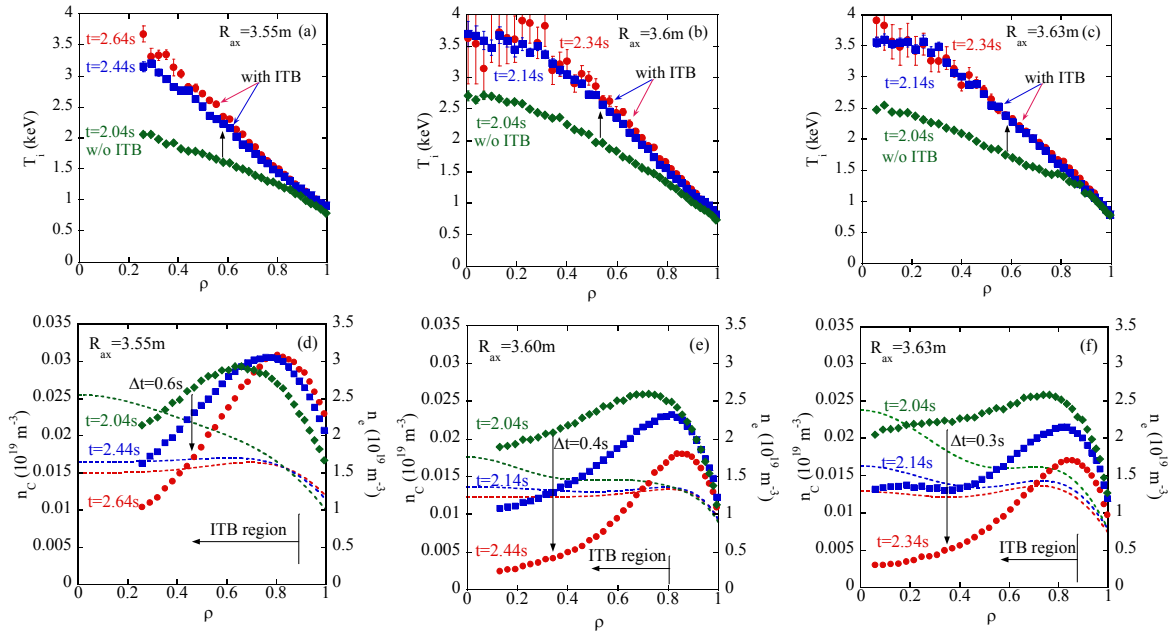
FIG.3. Radial profile of ion temperature in the plasma with (a) R_{ax}=3.55m , (b) 3.6m , and (c) 3.63m . Radial profile of carbon density in the plasma with (d) R_{ax}=3.55m , (e) 3.6m , and (f) 3.63m . Dashed lines in (d)-(f) shows the fitted line of electron density profile.
