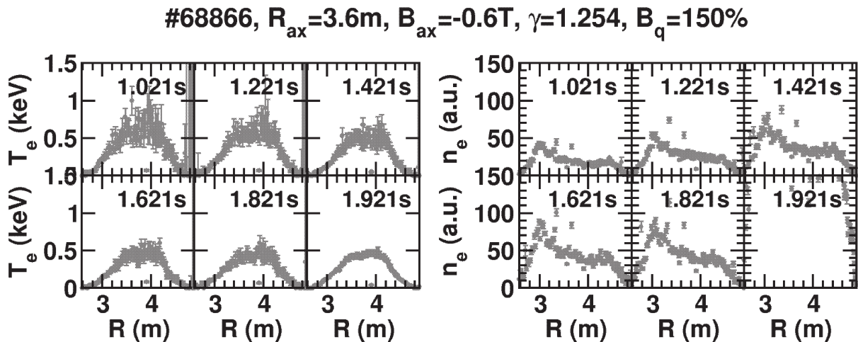
Fig. 1. Time evolutions of profiles of the electron temperature and density on the horizontal cross section at highest- \beta discharge. At t=1.921 [s], the fluttering of T_e profile was appeared.
