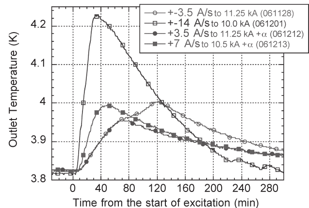
Fig. 2. Temperature rises at the outlet of helical coil by excitation, where the inlet temperature and the mass flow were 3.2 K and 50 g/s, respectively.
