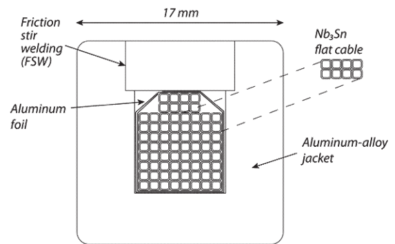
Fig. 1. 10-kA-class sub-scale superconductor developed for demonstration of aluminum-alloy jacketed conductors.
