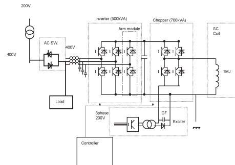
Figure 3: Circuit diagram of full-scale demo SMES.
