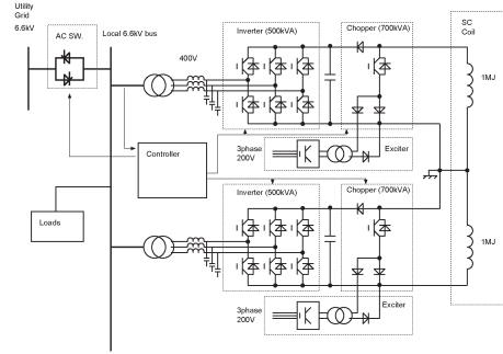
Figure 1: Circuit diagram of 1 MJ class SMES UPS.
