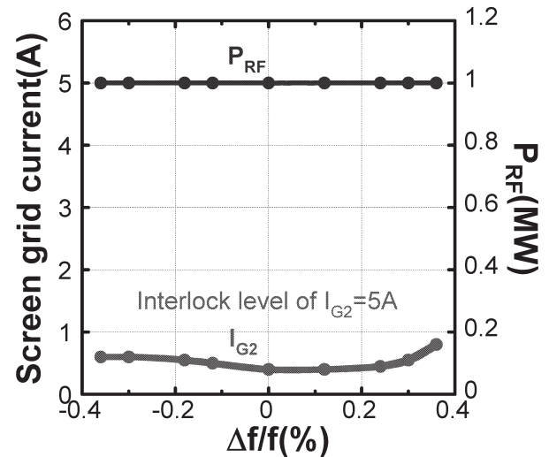
Fig.3 Dependence of screen grid current on frequency at RF output power of 1MW.
