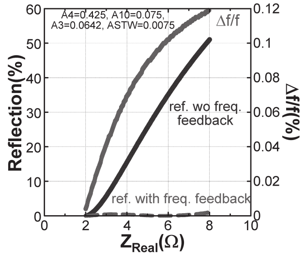
Fig.2 Reduction of reflected power fraction in the loading resistance range of 2\Omega to 8\Omega by changing frequency.
