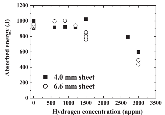
Fig. 2 Correlation between hydrogen concentration and impact strength at 173 K.
