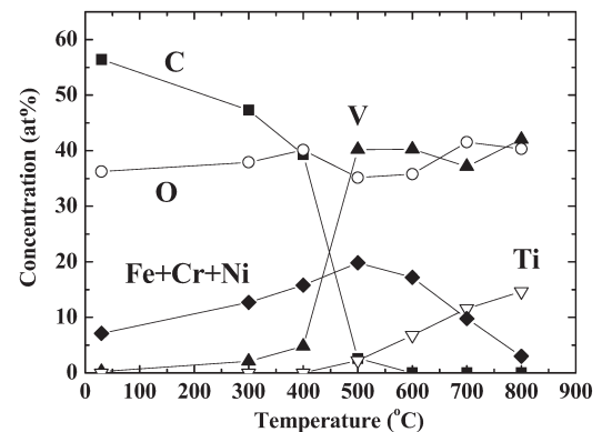
Fig. 1 Change in surface composition of V alloy specimen heated in vacuum after exposure to LHD plasma.
