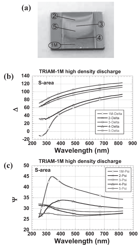
Fig.2 (a) Material specimen which was exposed to the long duration plasma in TRIAM-1M, (b) relative phase \Delta of p and s polarization and (c) relative amplitude \Psi of p and s polarization.
