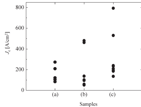
Fig. 1 Increase of J_c in the cylindrical bulks by composing with Ni meshes and intermediate pressing process. (a) without Ni meshes and intermediate pressing, (b) with Ni meshes and without intermediate pressing and (c) with Ni meshes and intermediate pressing and resintering process.
