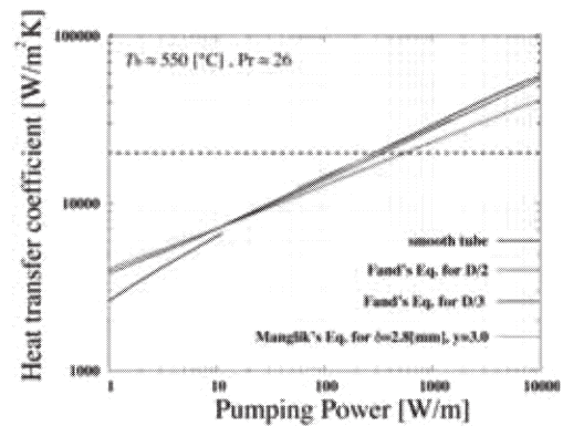
Fig. 3 Heat transfer performances for pumping power
