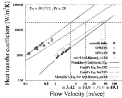
Fig. 2 Heat transfer performances for flow velocity
