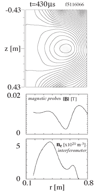
Fig. 2. Poloidal flux contour (top), radial profiles of magnetic field strength (middle) and electron density (bottom).
