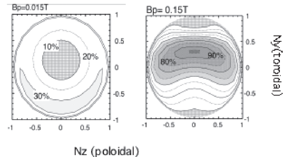
Fig. 3 Contours of conversion efficiency from incident EMW of the optimal polarization to EBW in N_y - N_z space.
