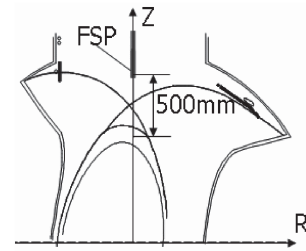
Fig. 1. Poloidal cross-sections of LHD plasma and vacuum vessel at the positions of the fast scanning Langmuir probe (FSP).
