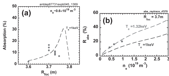
Fig. 1: Efficiency of absorbed power for 82.7GHz. (a) Antenna focal point on the equatorial plane R_{foc} dependence (closed circles) for the density of 0.6 \times 10^{19} m^{-3} . (b) Electron density dependence for R_{foc} = 3.7 m. The dashed lines show the calculation results by ray-tracing.
