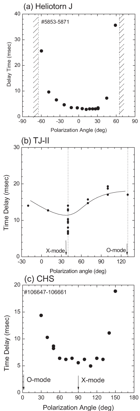
Fig. 1 Dependence of delay time for plasma breakdown on polarization of injected EC waves
