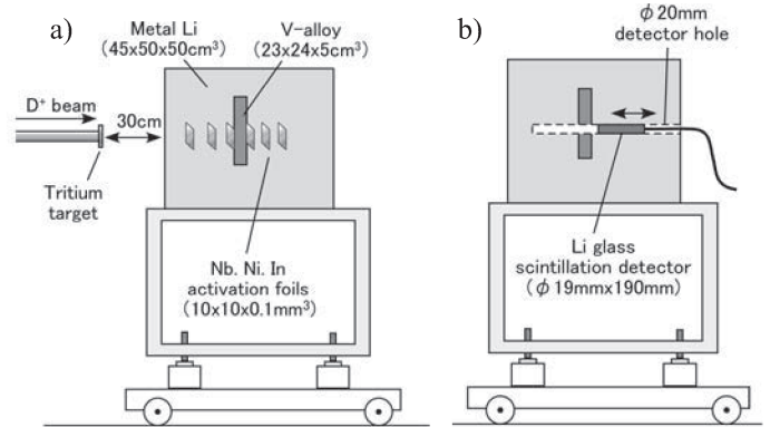
Fig. 1. Schematic drawing of a) reaction rate and b) tritium production rate measurements in Li/V-alloy assembly.
