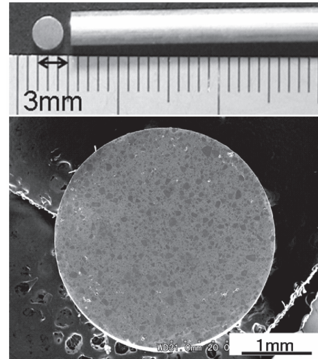
Fig.1 Macrostructure of the extruded wire 3 mm in diameter from the high- V_f \text{MgB}_2/\text{Al} composite material: (a) appearance of the extruded sample, and (b) SEM image of its cross section
