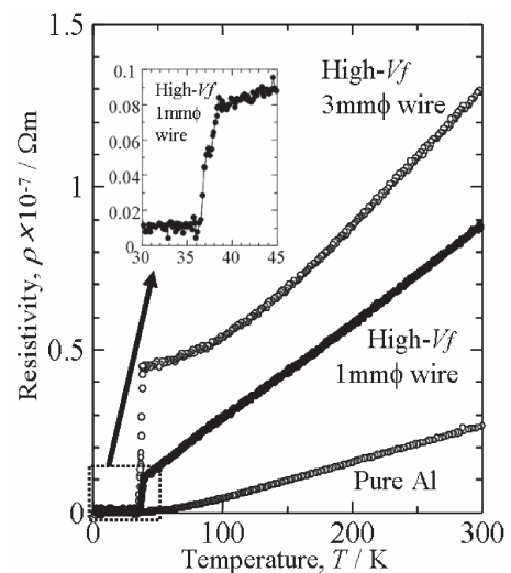
Fig.3 Temperature dependence of electrical resistivity of the extruded 3 and 1 mm high- V_f \text{MgB}_2/\text{Al} composite material wires and of the pure aluminium.
