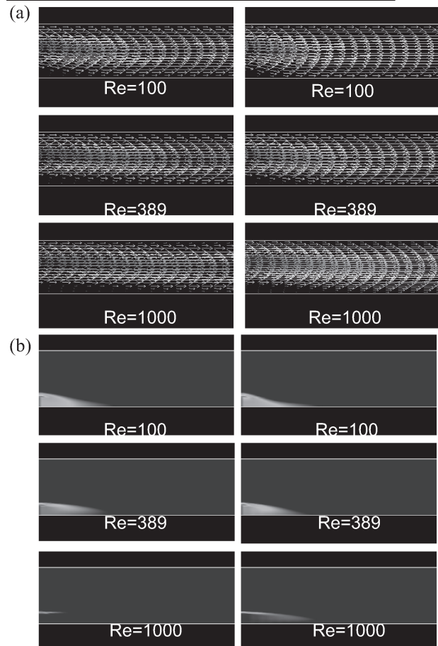
Figure 2 Two-dimensional velocity vector and temperature contour at Pr =7.1: (a)velocity vector, left hand side is non-MHD, right hand side is MHD, (b)temperature contour, left hand side is non-MHD, right hand side is MHD
