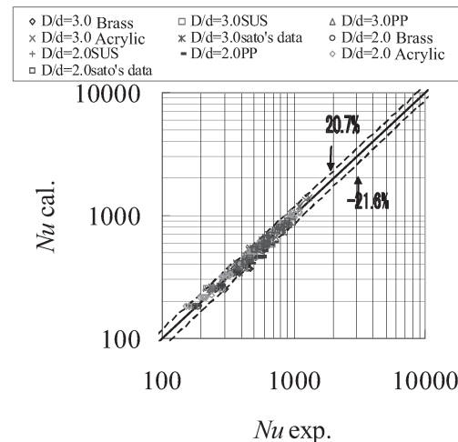
Fig. 2 Prediction of heat transfer performance of SPP
