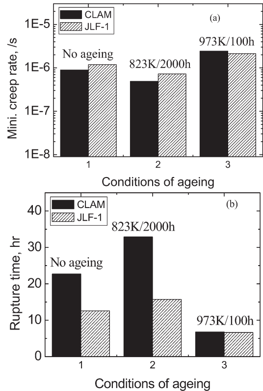
Fig. 2 Creep properties tested at 823 K / 250 MPa:
