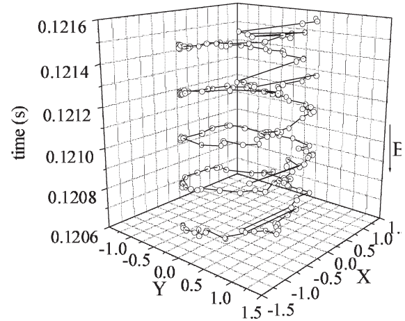
Fig. 2. Orbit of displacement in the cross section during ECH.
