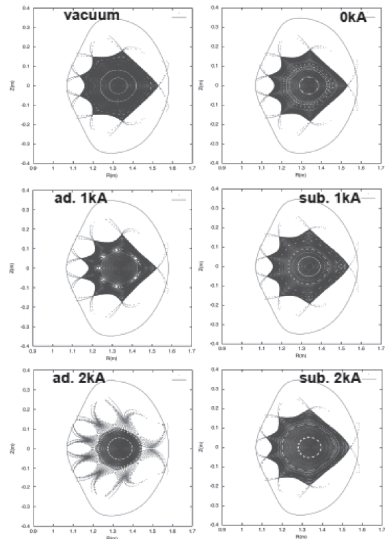
Fig.1. Puncture map of field lines on the standard configuration with net toroidal currents.
