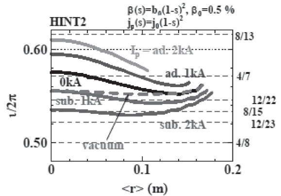
Fig.2. Profiles of the rotational transform of the standard configuration with net toroidal currents.
