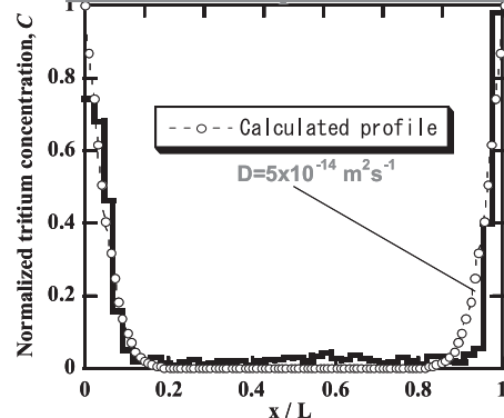
Fig.2 (a) Surface distribution and (b) diffusion profile by tritium for stainless steel exposed to gaseous T/H.
