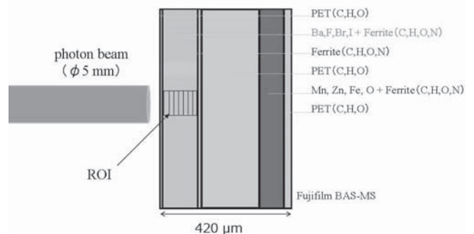
Fig. 2 Geometry of calculation
