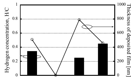
Fig.2. Hydrogen concentration and film thickness of co-deposited films on probes in a vicinity of helical divertor.
