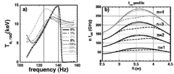
Fig. 2: a) Calculated ECE spectrum assuming T_{e,bulk} = 15 * (1 - \rho^2)^2 (keV) and T_{e,high} = 100 * (1 - \rho^2)^2 (keV) and n_e = 2.0 * (1 - \rho^8)^2 (\times 10^{18} m^{-3}) for various n_{e,high}/n_e . b) The dependence o the electron cyclotron and its harmonic frequencies along line of sight. Frequency down shift effect is shown for the electrons of the energy, E_0=15 keV and 100 keV electrons. Here, electron energy is assumed to depend on the minor radius as E_0(1 - \rho^2)^2 .
