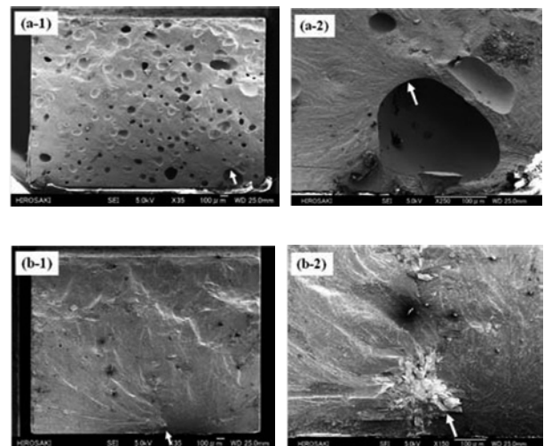
Fig. 1. (a-1) Fracture surface of a non-annealed specimen of a Dy123 porous bulk. (a-2) Magnified view around crack initiation site shown by an arrow in (a-1). (b-1) Fracture surface of a non-annealed specimen of a Dy123 low porosity bulk. (b-2) Magnified view around crack initiation site shown by an arrow in (b-1).
