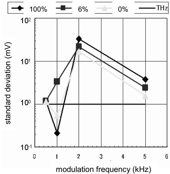
Fig. 2. Example of noise level measurement in the plasma discharge. The noise level is plotted as a function of center frequency of Lock-in amplifier. Excited laser power to PC antenna was changed; 100% (diamond), 6% (square), and 0% (triangle). Estimated radiated terahertz wave level is also plotted as a reference.
