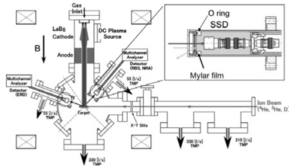
Fig. 1: Schematics of experimental device.
