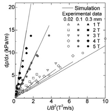
Fig. 2. Experimental (symbols) and simulated (lines) pressure drop
