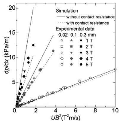
Fig. 3. Experimental (symbols) and simulated (lines) modified pressure drop
