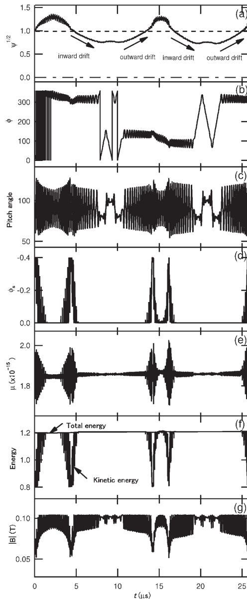
Fig. 1: Typical time evolutions of parameters of the injected electron.
