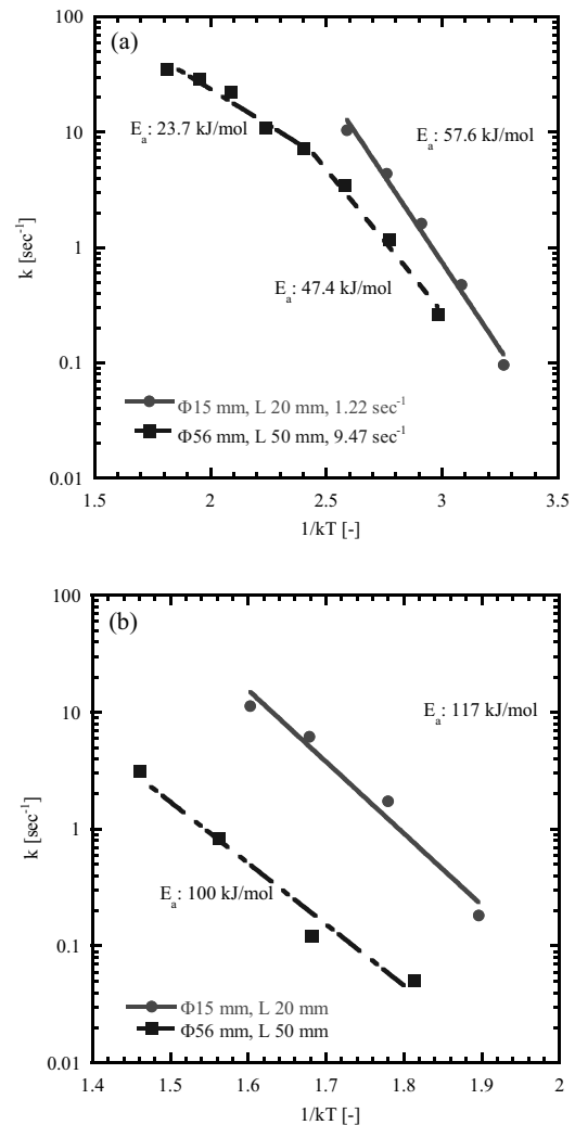
Fig. 1. Comparison of the Arrhenius plots of the oxidation performance between small- and large- size catalysts: (a). Hydrogen gas, (b). Methane gas
