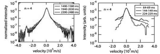
Fig. 2. Velocity distributions along the line of sight of the excited hydrogen atoms in the n = 4 state for the LHD plasma at t = 1490 - 1580 , 1940 - 2030 , and 2390 - 2480 ms (left) and those for the GAMMA10 plasma at t = 64 - 69 , 144 - 149 and 224 - 229 ms (right).
