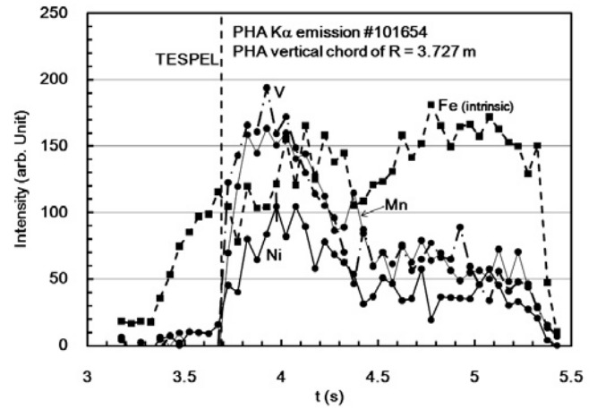
Fig.2 Temporal developments of K\alpha line intensities of the triple tracers: V, Mn and Ni in case of n_e (line average)= 4.8 \times 10^{19} \text{ m}^{-3} at t= 4.0 s. The emission of Fe as an intrinsic impurity shows different behavior from the tracers.
