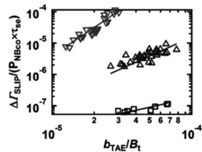
Fig.1 Dependence of loss fluxes on the relative TAE magnetic fluctuation amplitude at the magnetic probe in plasmas with R_{mag}=3.75 m(squares), 3.85 m(triangles) and 4.00 m(inversed triangles).
