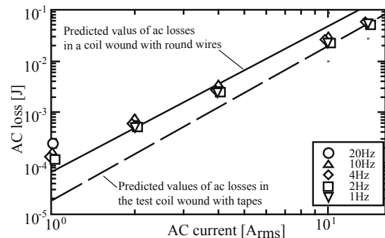
Fig. 1 AC loss properties of MgB 2 test coil wound with a parallel conductor.
