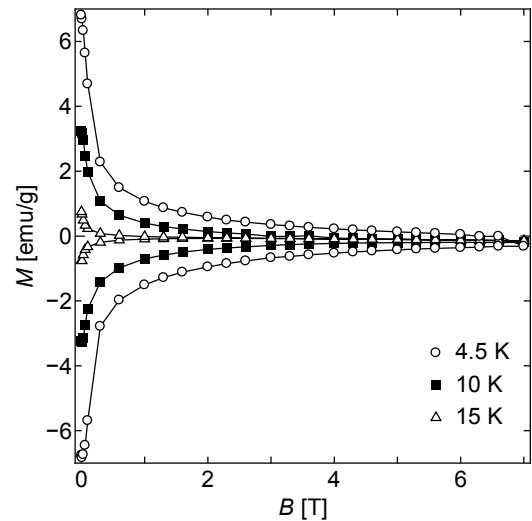
Fig. 1. Magnetization curve at 4.5-15 K.
