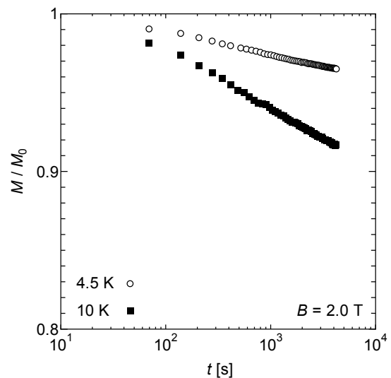
Fig. 2. relaxation of normalized magnetization at 2.0 T in 4.5K and 10K.
