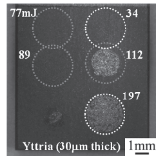
Fig. 1. Surface view of the coating layer on V-4Cr-4Ti-0.1Y-0.1Si alloy after laser shots of various energy.
